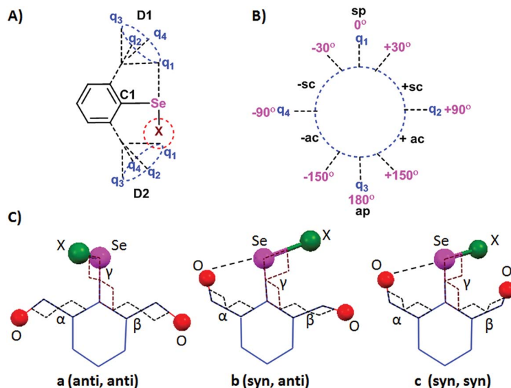
Fig. 11 (A) Rotational motion of D1 and D2. (B) Classification of the different torsion angles. (C) Three of the configurations of 2,6-disubstituted systems.
