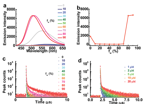
Fig. 3 (a) Steady-state emission spectra of 20 \mu\text{M} PXZT in THF and water mixtures at different f_w in air, \lambda_{\text{ex}} = 340 nm. (b) The emission intensity at 506 nm with the change of f_w , \lambda_{\text{ex}} = 340 nm. (c) Transient photoluminescence decay spectra of PXZT in THF/water mixtures with different f_w in air, \lambda_{\text{ex}} = 377 nm. (d) Transient photoluminescence decay spectra of different concentration of PXZT in THF/water mixtures ( f_w = 90 ) in air, \lambda_{\text{ex}} = 377 nm, \lambda_{\text{em}} = 506 nm.
