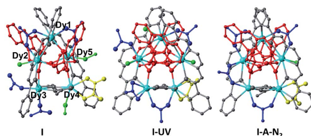
Fig. 2 The pentameric units in the structures of I, I-UV and I-A-N 2 . The common fragments (2EDDC 2− and 2 acetate) are shown in grey, Dy in cyan, other acetate in blue, C 15 H 11 PO 3 in red, oxalate in yellow, and H 2 O and CH 3 OH solvents in green.
