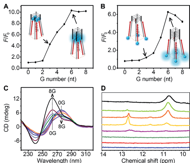
Fig. 4 Ratios of fluorescence peak intensity of (A) 1.0 \mu M O1-DTPE and (B) O1'-DTPE after and before ( F/F_0 ) hybridization with O1'-nG ( n = 0 to 8) in TE reaction buffer at 25 °C. (C) CD spectra of 20 \mu M O1'-nG ( n = 0 to 8) in TE reaction buffer at 25 °C. (D) 1 H-NMR spectra of O1'-nG ( n = 1 to 8 from bottom to top) in 10 mM phosphate buffer pH 7.4, with 100 mM NaCl and 10 mM MgCl 2 at 25 °C.
