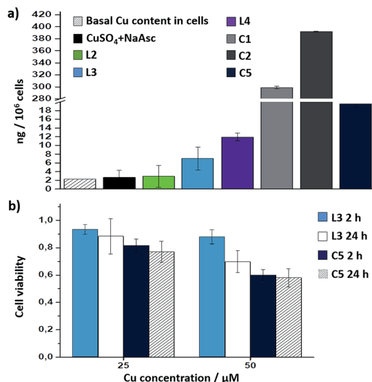
Fig. 5 (a) ICP-MS results of the intracellular accumulation of copper after incubation of cells in DMEM with 75 \mu M of copper complexes (in DMSO) for 2 h, double washing with PBS (2 \times 5 min) and digestion with HNO 3 . Note that when indicating L2, L3 or L4, the results refer to the copper accumulation using these ligands and NaAsc (standard conditions); (b) viability assays with in situ made Cu(I) complexes with L3, and with preformed C5 for 2 h and 24 h; the amount of viable cells was analysed by MTT assays.
