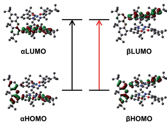
Fig. 9 Kohn-Sham molecular orbitals for the broken-symmetry solution ( S = 0 ) of [2^{*}]^{2+} associated with the calculated NIR transitions at 4995 and 3590 cm -1 . The predicted low energy bands are symmetric and antisymmetric linear combinations of the \alpha HOMO \rightarrow \alpha LUMO (black arrow), and \beta HOMO \rightarrow \beta LUMO (red arrow) local transitions on the individual salen radicals.
