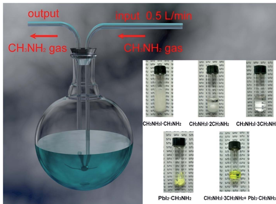
Fig. 13 Diagram of the \text{CH}_3\text{NH}_2 introduced \text{CH}_3\text{NH}_3\text{I} and \text{PbI}_2 powers and the mixture of \text{CH}_3\text{NH}_3\text{I}\cdot 3\text{CH}_3\text{NH}_2 and \text{PbI}_2\cdot\text{CH}_3\text{NH}_2 . 36
