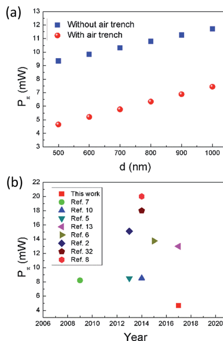
Fig. 8 (a) P_\pi as function of d with and without air trench. (b) Summarization of P_\pi reported in references.
