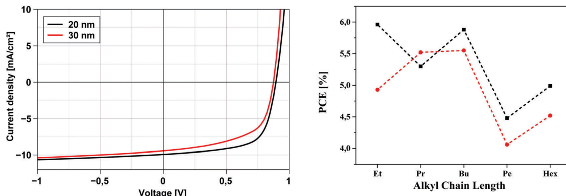
Fig. 6 J–V characteristics of heteropentacene 6b : C 60 (2 : 1) in m–i–p bulk-heterojunction solar cells with an active layer thickness of 20 nm and 30 nm as example (left) and power conversion efficiency (PCE) versus alkyl side chain length (black line 20 nm thickness, red line 30 nm) of all heteropentacenes 6b–f : C 60 (2 : 1) (right).
