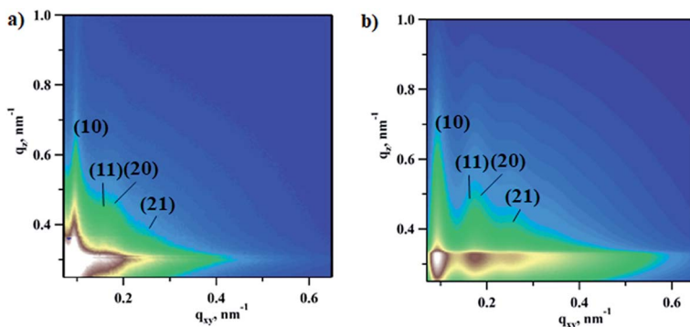
Fig. 2 Experimental (a) vs. fitted (b) 2D GISAXS images during carbon monoxide oxidation reaction with a CO to O 2 ratio of 2 : 1. Diffuse Kiessig fringes are typical of a NP monolayer with a well defined height. The fitting was performed in the BornAgain package using bimodal spheres submerged into a SiO 2 /Si substrate.
