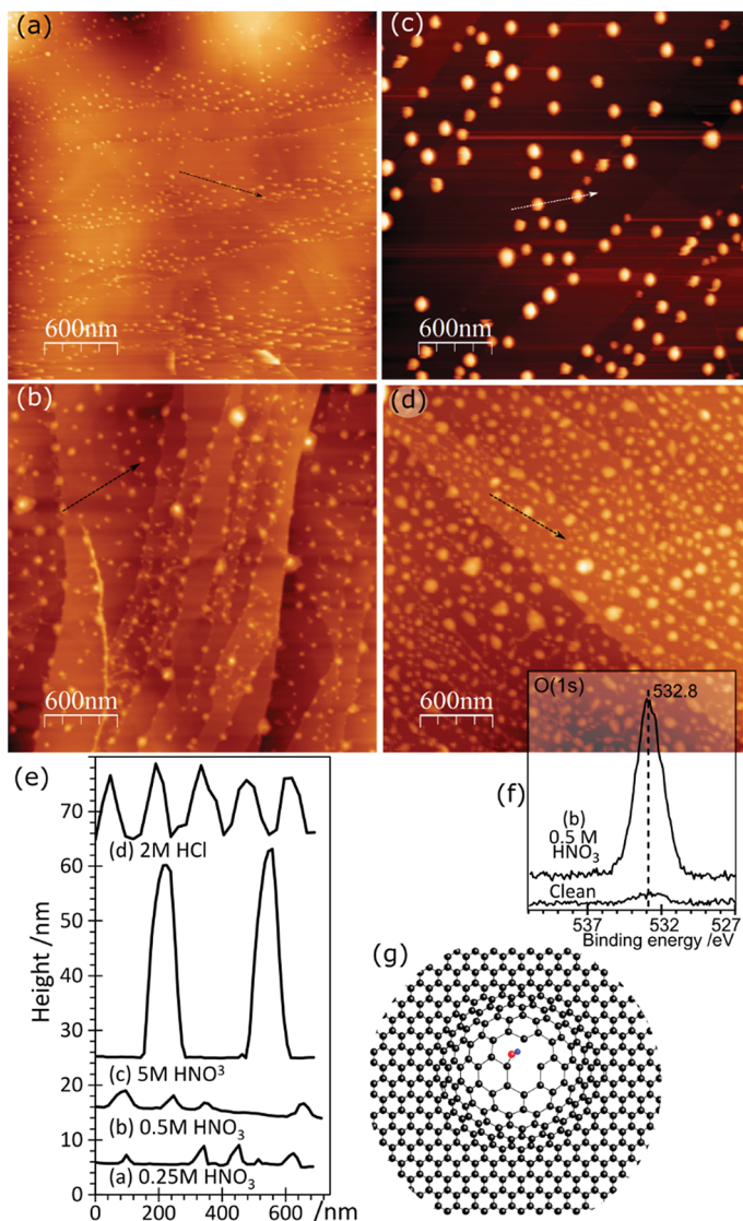
Fig. 1 AFM images showing the effect of different acid treatments on HOPG surfaces: (a) 0.25 M HNO 3 ; (b) 0.5 M HNO 3 ; (c) 5.0 M HNO 3 ; (d) 2.0 M HCl; (e) corresponding line profiles; (f) XPS spectrum of (1s) region from image (b); (g) model previously proposed 7 to account for AFM features in which functionalisation of existing defects in the lattice leads to a local delamination.
