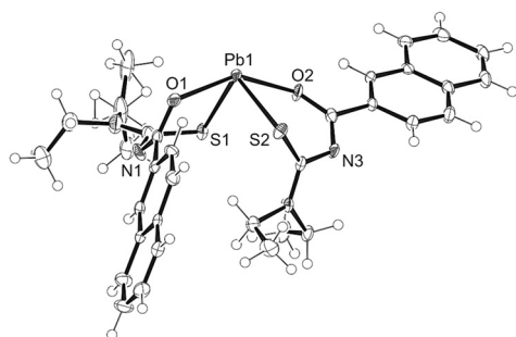
Fig. 1 A thermal ellipsoid plot representing the structure of 4. CCDC ref. 1005699.†
