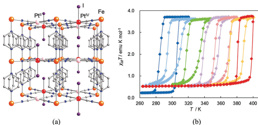
Fig. 21 (a) Crystal structure of {Fe(pz)[Pt(II/IV)(CN)4(I)]}. Atoms: Fe (orange), Pt II (pink), Pt IV (red), I (purple), C (gray), N (blue). (b) Magnetic behavior of {Fe(pz)[Pt(CN)4(I) n ]} n = 0.0 (blue); 0.1 (sky blue); 0.3 (green); 0.5 (violet); 0.7 (pink); 0.9 (orange); 1.0 (red). Reprinted with permission from ref. 68, Copyright 2011 American Chemical Society.
