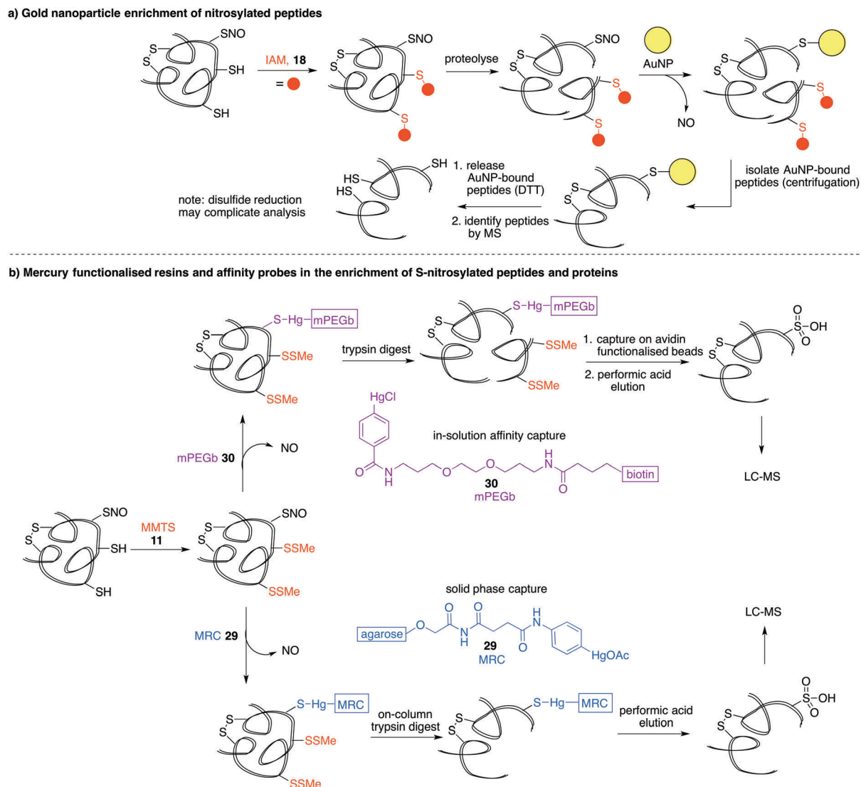
Fig. 6 (a) Gold nanoparticle (AuNP) capture of protein-SNO. Free thiols are blocked by iodoacetamide (IAM, 18 ), proteolysed, and trapped on AuNPs with release of NO. The AuNP-bound peptides are isolated and released by DTT reduction. (b) Organomercury capture of protein-SNO using either affinity capture (mPEGb, 30 ) or mercury resin bound capture (MRC, 29 ). Both methods require blocking of free thiols (by MMTS 11 , for instance), with performic acid elution to remove the captured peptides for analysis by mass spectrometry.
