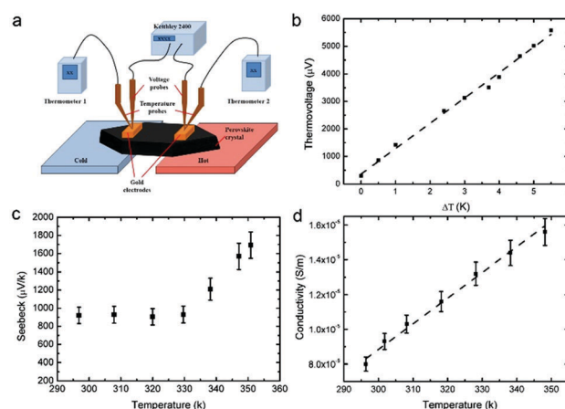
Fig. 3 Thermoelectric property characterization of the perovskite single crystal. (a) Schematic graph of the thermoelectric property measurement. (b) Thermal voltages at different applied temperature differences. The Seebeck coefficient can be obtained from the linear fit (dashed lines); (c) Seebeck coefficients at different average temperatures; (d) conductivity at different temperatures and the dashed line is the linear fit.
