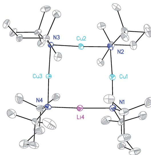
Fig. 3 Molecular structure of 9 (30% probability and with H-atoms omitted, major metal occupancies shown). Selected bond lengths (Å): N1–M1 1.953(3) , N2–M1 1.973(3) , N2–M2 1.931(3) , N3–M2 1.922(3) , N3–M3 1.961(3) , N4–M3 1.955(3) , N4–M4 2.001(4) , N1–M4 2.018(4) .
