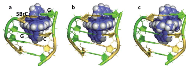
Fig. 5 The DNA tetramer d((5BrC)GGC/GCCG) with the complexes (a) \Lambda - [\text{Ru}(\text{bpy})_2\text{dppz}]^{2+} (5LFS); (b) \Lambda - [\text{Ru}(\text{phen})_2\text{dppz}]^{2+} (5LFW); (c) \Lambda - [\text{Ru}(\text{phen})_2 11,12\text{-dimethyldppz}]^{2+} (5LFX). 30
