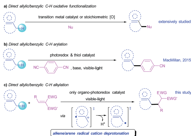
Scheme 1 Direct functionalization of allylic/benzylic \text{sp}^3 C–H bonds.
