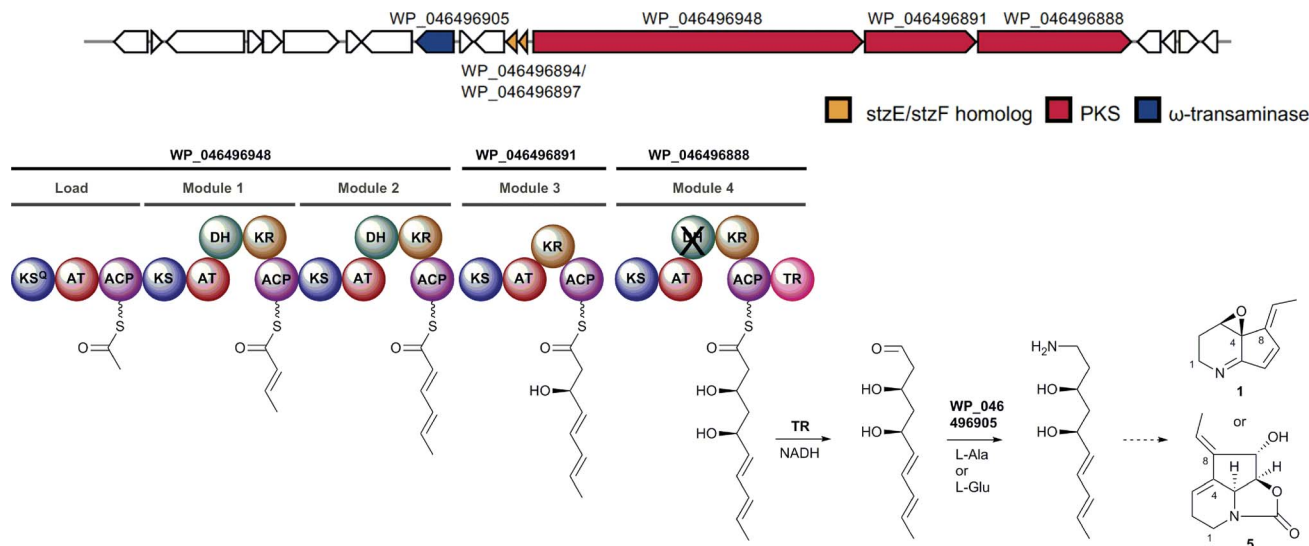
Fig. 6 Example of a putative polyketide alkaloid biosynthetic gene cluster identified in Streptomyces sp. NRRL-B24891. Based on the predicted structure of the chain assembled by the PKS and the presence of two genes encoding homologs of the StzE and StzF enzymes, the cluster is hypothesized to direct the biosynthesis of latumcidin 1 , streptazolin 5 or a structurally-related metabolite.
