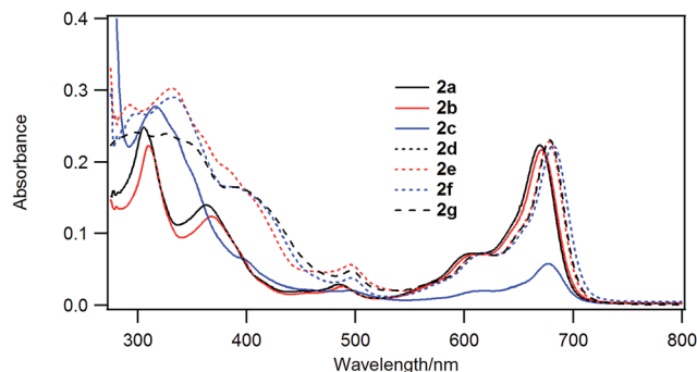
Fig. 3 UV-visible spectra of 2a (black solid line), 2b (red solid line), 2c (blue solid line), 2d (black dotted line), 2e (red dotted line), 2f (blue dotted line), and 2g (black dashed line). The concentration of 2a , 2b and 2d–g was 2 \times 10^{-6} M in dichloromethane. Visible spectra of 2c was the spectra of saturated dichloromethane solution.
