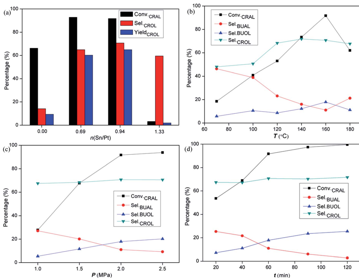
Fig. 8 (a) Liquid phase hydrogenation results over the \text{PtSn}_x/\text{LOC} catalysts with different Sn/Pt molar ratios. Reaction conditions: 1 mL CRAL catalyzed by 100 mg of the catalyst in 19 mL ethanol, T = 160 ^{\circ}\text{C} , p = 2.0 \text{ MPa} , t = 60 \text{ min} . Liquid phase hydrogenation results of CRAL over the \text{PtSn}_{0.94}/\text{LOC} as a function of: (b) temperature, (c) \text{H}_2 pressure and (d) time.
