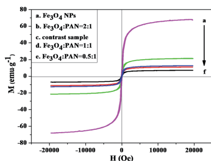
Fig. 12 Hysteresis loops of the \text{Fe}_3\text{O}_4 NPs, the heterogeneous nanofiber yarns with different mass ratios of \text{Fe}_3\text{O}_4 NPs and of the homogeneous nanofiber yarns (contrast sample).
