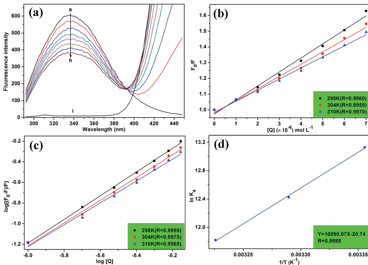
Fig. 1 (a) Fluorescence spectra of HSA ( 2.0 \times 10^{-6} mol L -1 ) in the absence and presence of MOXH at 298 K. MOXH concentrations (a–h) were 0, 1.0, 2.0, 3.0, 4.0, 5.0, 6.0, and 7.0 \times 10^{-6} mol L -1 . Curve i shows the emission spectrum of MOXH alone ( 7.0 \times 10^{-6} mol L -1 ). (b) Stern–Volmer plots for MOXH interacting with HSA at three different temperatures. (c) Plot of \log[(F_0 - F)/F] versus \log[Q] for the MOXH–HSA system at three different temperatures. (d) van't Hoff plot of the MOXH–HSA system.
