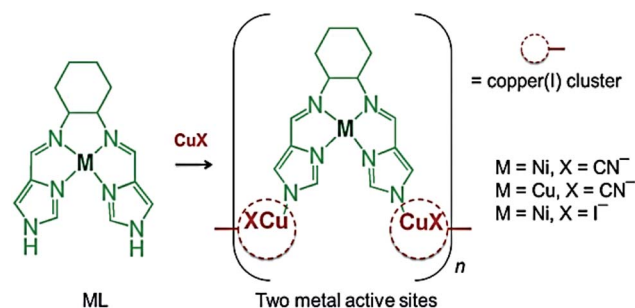
Scheme 3 Synthesis of [\text{NiL}]_2[\text{Cu}(\text{i})\text{CN}]_9_n , [\text{Cu}(\text{ii})\text{L}]_2[\text{Cu}(\text{i})\text{CN}]_9_n and [\text{NiL}][\text{Cu}(\text{i})\text{I}]_2_n . [Reproduced from ref. 101 with permission from The Royal Society of Chemistry.]
