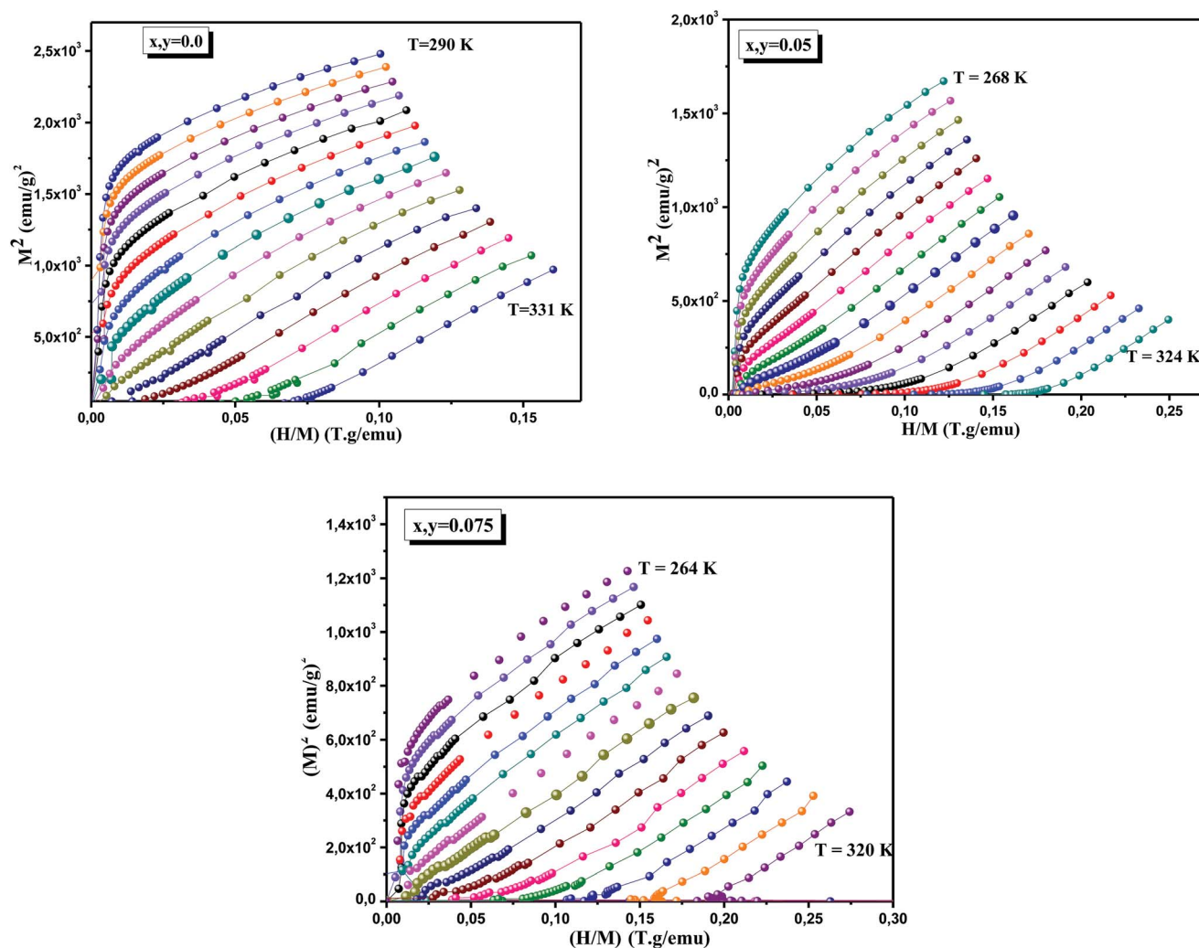
Fig. 5 Arrott plots around T_C for \text{La}_{0.7}\text{Ca}_{0.1}\text{Pb}_{0.2}\text{Mn}_{1-x-y}\text{Al}_x\text{Sn}_y\text{O}_3 ( x, y = 0.0, 0.05 and 0.075 ) samples. According to the mean field model, values of critical exponents \beta = 0.5 and \gamma = 1 should generate the regular Arrott plots, M^2 vs. \mu_0 H/M .
