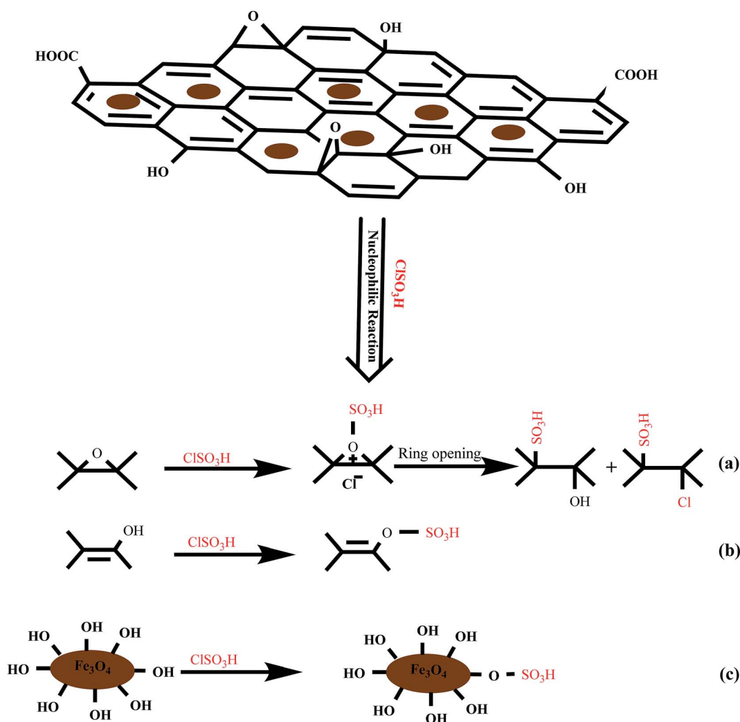
Scheme 1 Proposed nucleophilic substitution reactions for modification of magnetic graphene oxide by chlorosulphonic acid.
