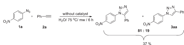
Scheme 1 AAC reaction of 1-azido-4-nitrobenzene 1a and phenylacetylene 2a without the catalyst.
