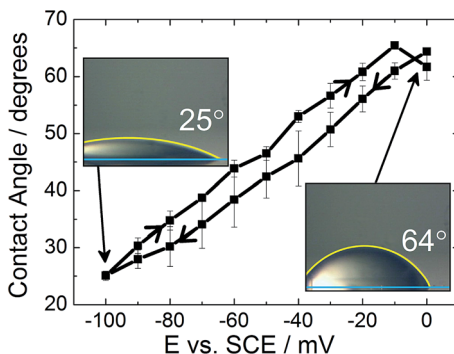
Fig. 2 Electrowetting response for a dichloroethane droplet on mercury surrounded by 0.10 \text{ mol dm}^{-3} LiCl.
