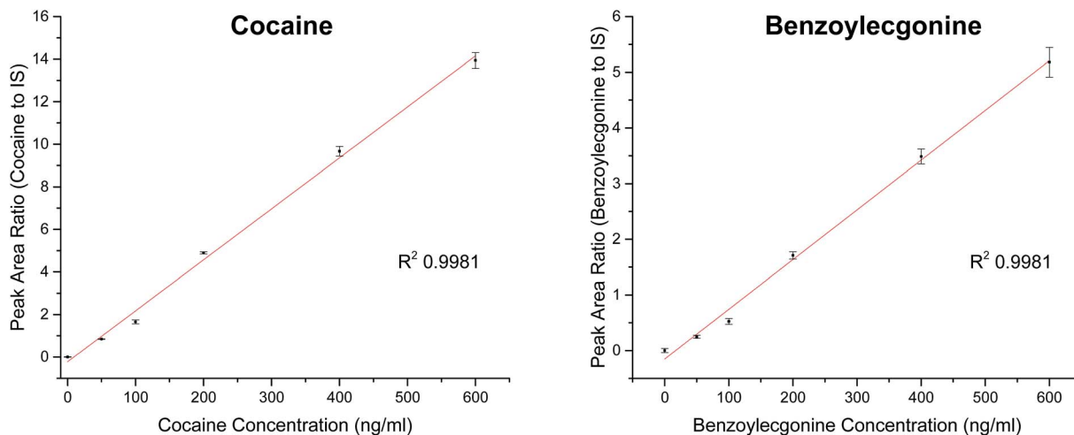
Fig. 5 Calibration curve for cocaine ( m/z 304) and benzoylecgonine ( m/z 290) in pooled oral fluid analysed using Plate Express™ with an expression compact mass spectrometer (CMS) with cocaine- d_7 ( m/z 185) internal standard.
