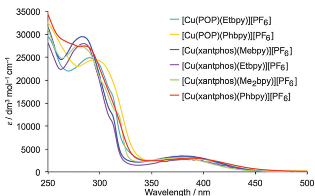
Fig. 7 Solution absorption spectra of the [Cu(P^P)(N^N)][PF 6 ] 2 complexes (CH 2 Cl 2 , 2.5 × 10 -5 mol dm -3 ).
