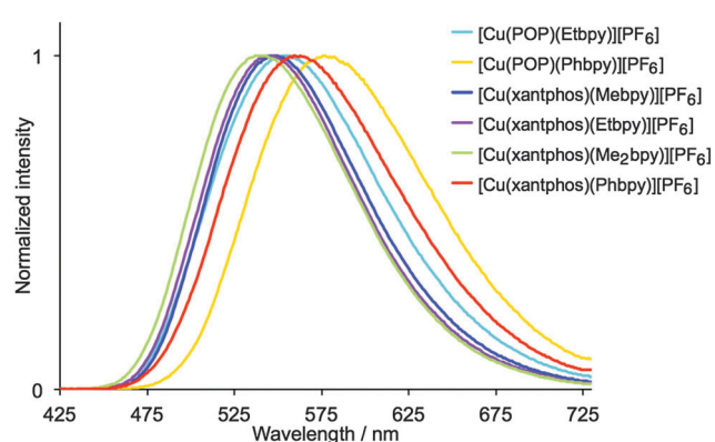
Fig. 8 Normalized emission spectra of solid [Cu(P^P)(N^N)][PF 6 ] 2 . For λ exc , see Table 1.
