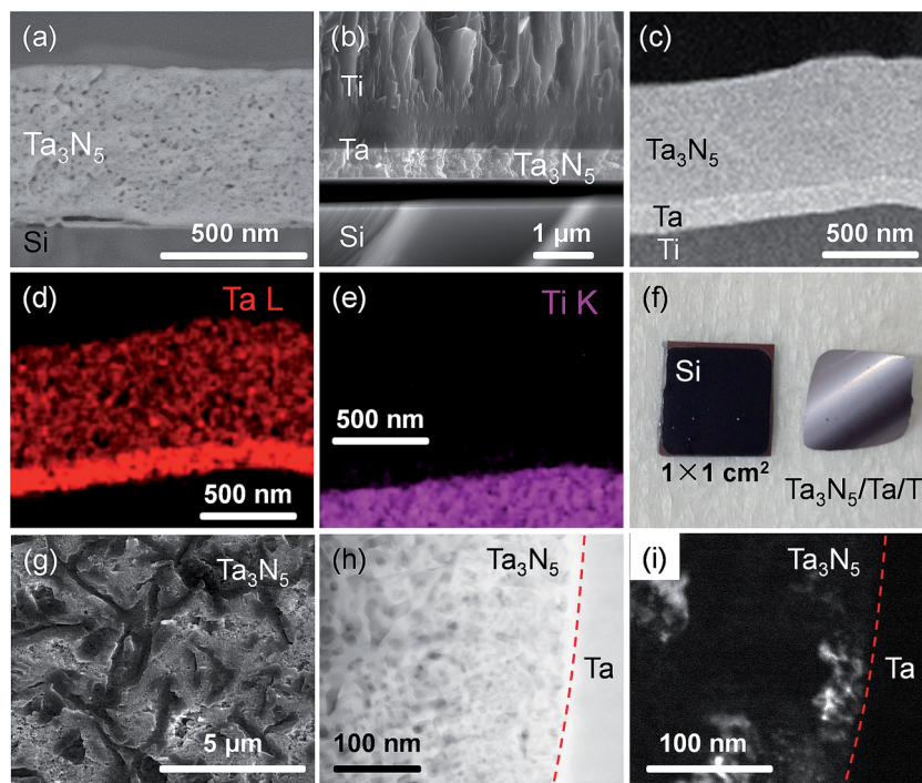
Fig. 3 Cross-sectional SEM images of (a) \text{Ta}_3\text{N}_5/\text{Si} and (b) \text{Ti-Ta-Ta}_3\text{N}_5/\text{Si} , (c) cross-sectional STEM image of transferred \text{Ta}_3\text{N}_5/\text{Ta/Ti} , EDS maps for (d) Ta and (e) Ti taken from the STEM image in panel (c), (f) digital photographs of a \text{Ta}_3\text{N}_5/\text{Ta/Ti} sample transferred from a Si substrate, (g) top-view SEM image of a \text{Ta}_3\text{N}_5/\text{Ta/Ti} sample, and dark-field (h) STEM and (i) zone-axis TEM images of a \text{Ta}_3\text{N}_5/\text{Ta/Ti} sample near the \text{Ta}_3\text{N}_5/\text{Ta} interface.
