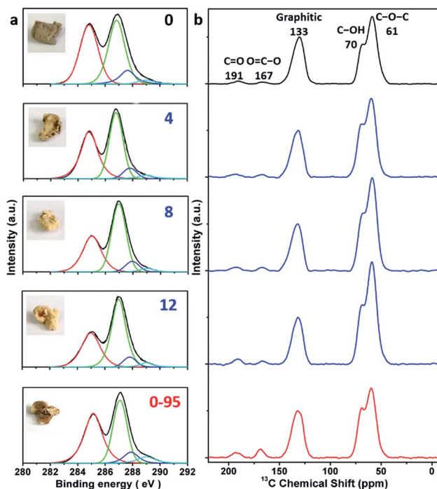
Fig. 1 (a) C 1s XPS spectra and photographs (inset), and (b) magic-angle spinning ^{13}\text{C} ssNMR spectra of different freeze-dried GO- n and GO-0-95 samples; the values of n are depicted in (a).
