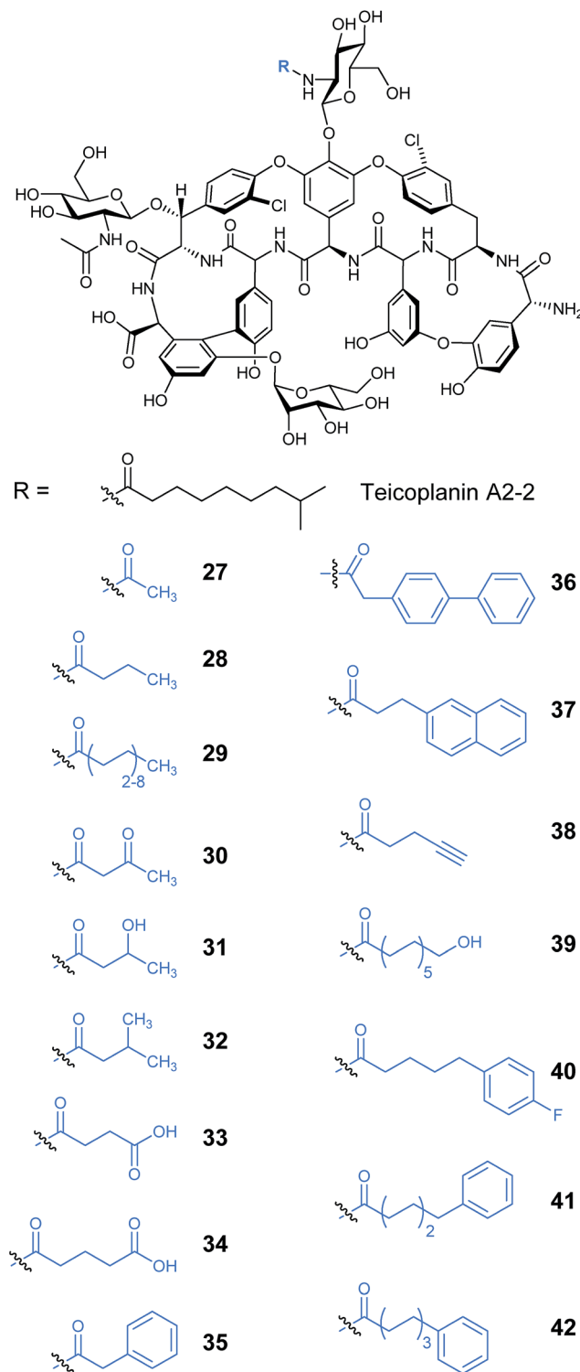
Fig. 10 Produced mono-acylated teicoplanin A2-2 analogues. 41
