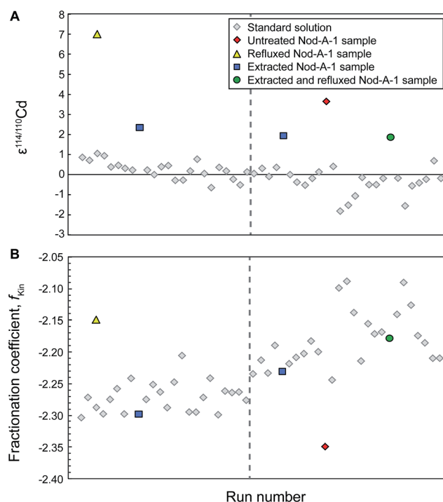
Fig. 2 Typical analytical session of repeat measurements of the NIST SRM 3108 Cd standard solution doped with Cd double spike together with interspersed measurements of the ferromanganese nodule Nod-A-1 that passed through both stages of column chemistry and were subsequently extracted and/or refluxed to remove the organic residue, or left untreated. The dashed grey line indicates when the sweep gas of the desolvating sample introduction system was adjusted; this typically leads to a change in the instrumental mass bias. All samples of Nod-A-1 should yield identical isotope compositions (A). For this particular instrument session, samples that were cleaned by extraction or extraction and refluxing give \epsilon^{114/110}\text{Cd} = 2.1 \pm 0.4 (2SD), whilst the untreated and particularly the refluxed samples have much higher \epsilon^{114/110}\text{Cd} values. Note the delayed 2\epsilon shift in the isotope data for the NIST Cd standards that were analyzed following the untreated sample. The shift occurs only with the second standard analyses after the sample and the instrumental fractionation coefficient f_{\text{kin}} does not display a simple step change after this analysis (B).
