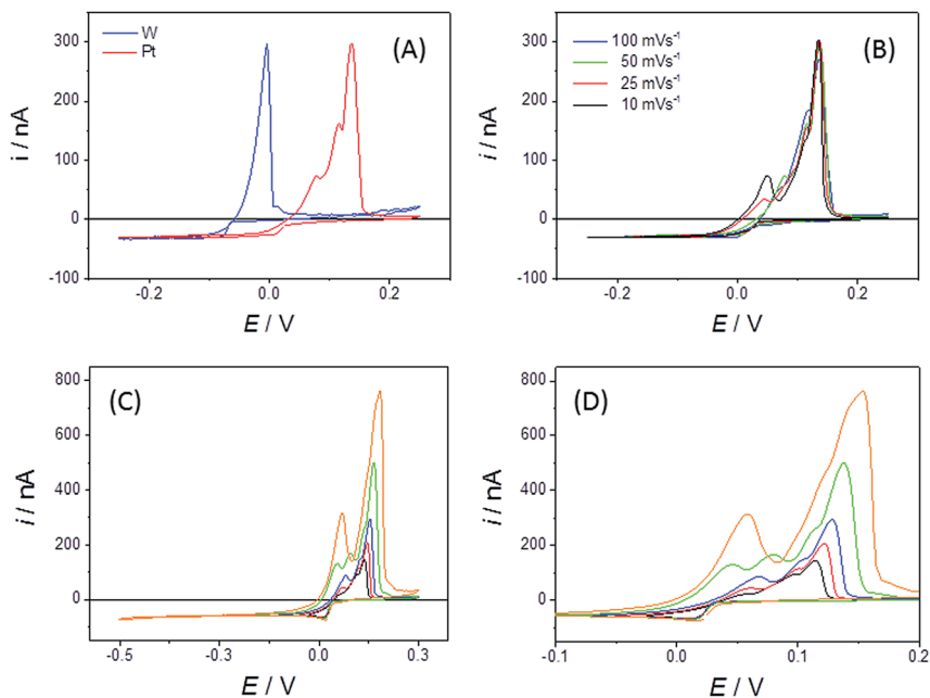
Fig. 7 (A) CVs recorded using a sweep rate of 50\text{ mV s}^{-1} with an r = 25\text{ }\mu\text{m} Pt and an r = 25\text{ }\mu\text{m} W MSM in LKE + 1.6\text{ mM BiCl}_3 at 668\text{ K} . (B) CVs recorded at the given sweep rates using an r = 15\text{ }\mu\text{m} diameter Pt MSM in LKE + 5\text{ mM BiCl}_3 at 690\text{ K} . (C) CV and (D) expanded section of the CV at 50\text{ mV s}^{-1} with a progressively increasing negative potential limit recorded using a Pt MSM ( r = 25\text{ }\mu\text{m} ) in LKE + 1.6\text{ mM BiCl}_3 .
