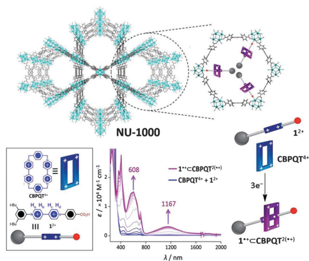
Fig. 5 Schematic of NU-1000 containing the semirotaxane (top). Representation of the semirotaxane components 1 2+ and CBPQT 4+ (bottom left). Reduction of 1 2+ and CBPQT 4+ with 3 mol e - generates the semirotaxane 1 + < CBPQT 2(+) (bottom right and centre where the redox-dependent absorption spectrum is shown). Reproduced from ref. 148 with permission from National Academy of Sciences, USA.
