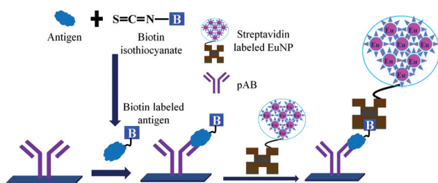
Fig. 14 Use of europium nanoparticles for the detection of PSA.
