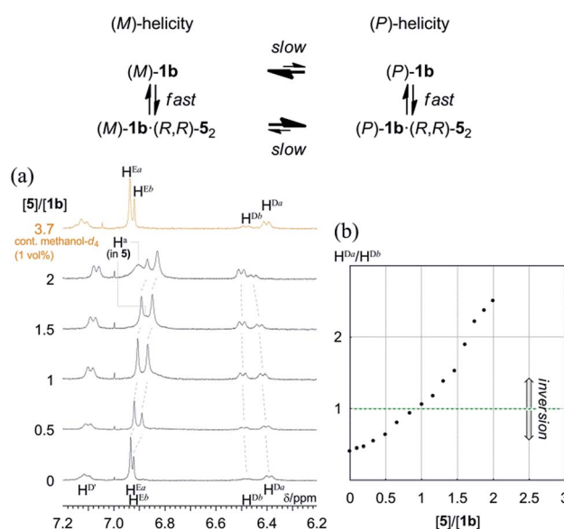
Fig. 10 (a) ^1\text{H} NMR spectra of ( R,R,R,R )- 1b (1 mM) in the presence of ( R,R )- 5 (0–2 equiv., and 3.7 equiv. containing 1 vol% methanol- d_4 ). All spectra were measured in \text{CDCl}_3 at 293 K. (b) Plot of the ratio of the populations of two species with ( M )- or ( P )-helicity versus equivalents of 5 added, based on phenylene protons \text{H}^{\text{Da}} and \text{H}^{\text{Db}} .
