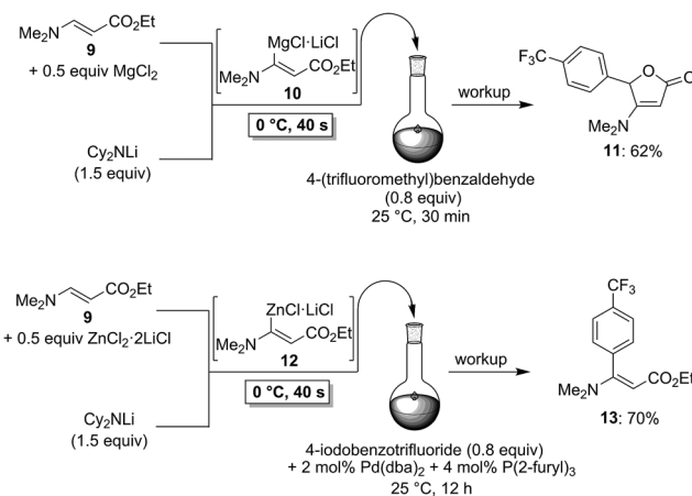
Scheme 4 In situ trapping magnesianation and zincation of ( E )-ethyl 3-(dimethylamino)acrylate ( 9 ) using Cy 2 NLI in a flow reactor.
