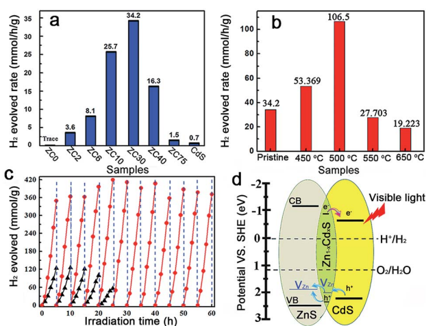
Fig. 3 (a) Photocatalytic \text{H}_2 -production activities of the ZCX samples and (b) ZC30 post-annealed at different temperatures in a 0.35 M \text{Na}_2\text{S} and 0.25 M \text{Na}_2\text{SO}_3 mixed aqueous solution under visible-light irradiation. (c) Comparison of the photocatalytic stabilities of pristine ZC30 (triangle) and ZC30-500 (circle). (d) Schematic illustrating charge transfer and separation in \text{ZnS}/\text{Zn}_{1-x}\text{Cd}_x\text{S}/\text{CdS} .
