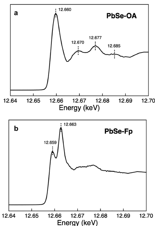
Fig. 5 Se XAS evidencing significant surface distortions in PbSe-Fp. (a) Se K-edge XAS of PbSe-OA. (b) Se K-edge XAS of PbSe-Fp.
