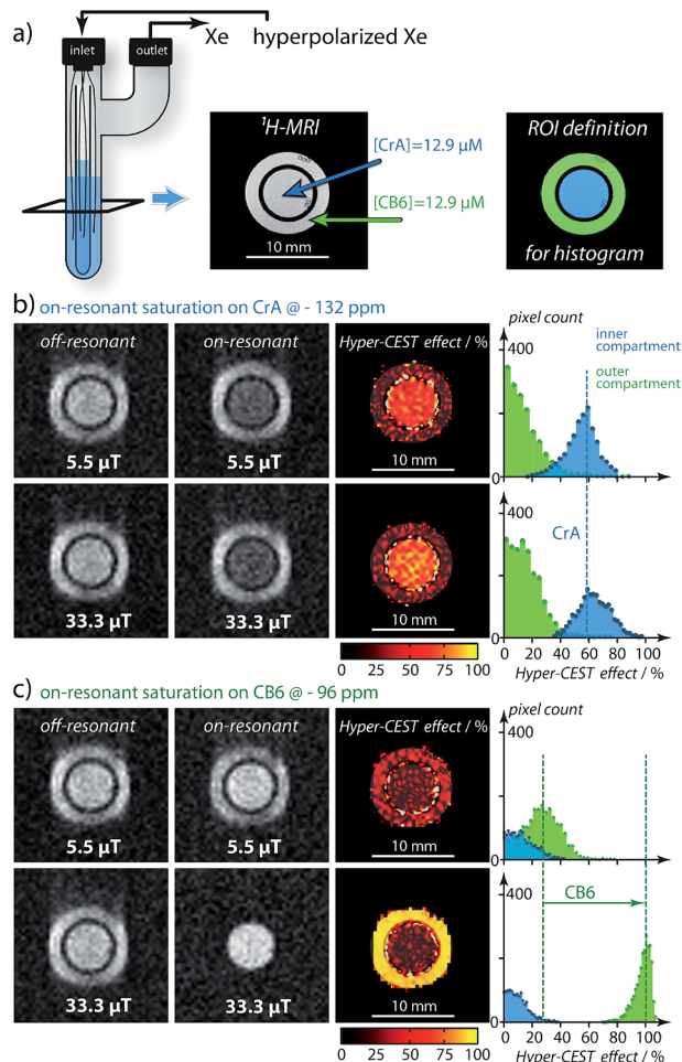
Fig. 3 Hyper-CEST effect mapping for equal concentrations of [CB6] = [CrA] = 12.9 \mu M in water at T = 295 K . (a) shows the proton ( ^1H )-MRI as a cross-section (tilted black square) of the double bubbling phantom and the region-of-interest (ROI) definition for histogram analysis. (b) Hyper-CEST effect maps of CrA for 5.5 \mu T ("low RF exposure") and 33.3 \mu T ("high RF exposure") both for 2 s of cw saturation calculated as the difference of the on-resonant image (saturation at -132 ppm) and the off-resonant image (saturation at +132 ppm) with respect to the free Xe in solution resonance. The Hyper-CEST effect of 60 % for both RF exposures is significant but unchanged. (c) CB6 Hyper-CEST effect maps for identical RF exposure but the on-resonant image (saturation at -96 ppm) and the off-resonant image (saturation at +96 ppm) with respect to the free Xe in solution resonance. Whereas the Hyper-CEST effect for 5.5 \mu T saturation strength was below 30 %, the stronger saturation resulted in \sim 100 % Hyper-CEST effect, thus revealing significantly higher gas turnover for the Xe–CB6 complex. The Xe–MR images were acquired with 64^2 resolution and cubic spline interpolated to 256^2 . The slight blurring in phase encoding direction originated from faster T_2 relaxation with CB6 in the outer compartment.
