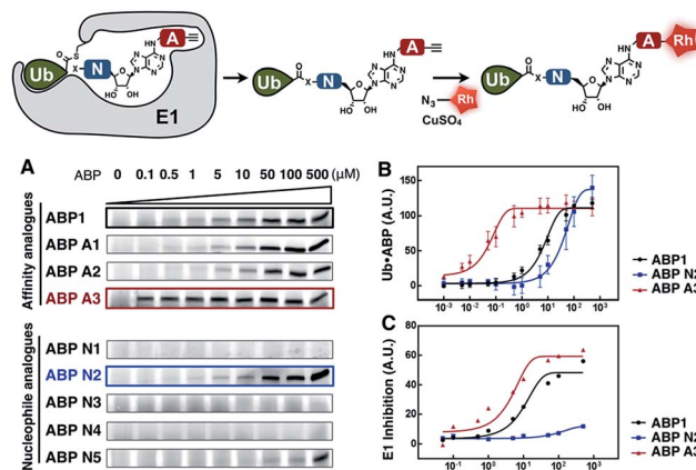
Fig. 4 (A) Dose dependent formation of Ub-ABP covalent adducts in the presence of UBE1 (0.5 μM), ATP (50 μM) and Ub (50 μM), after 2 hours at r.t. (B) The labeling efficiency of ABP1, ABP N2 and ABP A3 was compared via the quantification of the Ub-ABP levels at different concentrations. Each data point is shown as a triplicate (C) The inhibition potency of protein ubiquitination by ABP1, ABP N2 and ABP A3 was plotted based on the fluorescence intensity ratio of ubiquitin-modified GFP-Sic60 to total GFP-Sic60.
