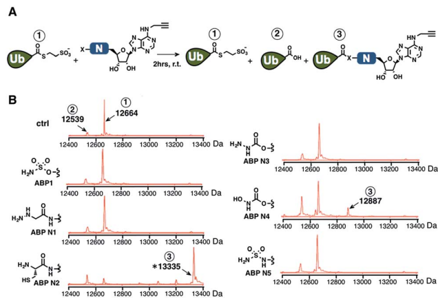
Fig. 3 (A) Schematic description of the intrinsic reactivity test of the nucleophile analogues using pre-activated ubiquitin thioester Ub-MES. (B) Deconvoluted mass spectra of the Ub-MES (100 μM) and ABP (1 mM) reaction mixture, after 2 hours of incubation at r.t. Reaction products are labeled as follows (1) Ub-MES, (2) ubiquitin, the hydrolysis product of Ub-MES, (3) Ub-ABP. * Ub-ABP N2 formed disulfide bond with free ABP N2, which was reduced to Ub-ABP N2 in the presence of TCEP (Fig. S1†).
