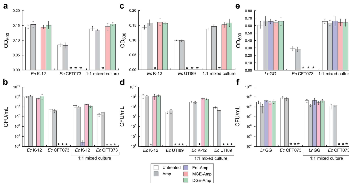
Fig. 5 MGE/DGE–Amp selectively kill uropathogenic E. coli in the presence of non-pathogenic E. coli K-12 and the probiotic L. rhamnosus GG. (a and b) Bacterial growth monitored by (a) OD_{600} and (b) CFU\ mL^{-1} for cultures of E. coli K-12 only, CFT073 only, and 1 : 1 K-12/CFT073 mixtures treated with 100 nM Amp or 100 nM (Glc)Ent–Amp 5/7/9 in the presence of 200 \mu M DP. (c and d) Bacterial growth monitored by (c) OD_{600} and (d) CFU\ mL^{-1} for cultures of E. coli K-12 only, UTI89 only, and 1 : 1 K-12/UTI89 mixtures treated with 100 nM Amp or 100 nM (Glc)Ent–Amp 5/7/9 in the presence of 200 \mu M DP. (e and f) Bacterial growth monitored by (e) OD_{600} and (f) CFU\ mL^{-1} for cultures of L. rhamnosus GG only, E. coli CFT073 only, and 1 : 1 L. rhamnosus GG/ E. coli CFT073 mixtures treated with 1 \mu M Amp or 1 \mu M (Glc)Ent–Amp 5/7/9 in the presence of 200 \mu M DP. All mixed- E. coli antimicrobial assays were performed in 50% MHB medium and all mixed-species antimicrobial assays were conducted in 1 : 1 MRS/MHB medium ( t = 19\ h , T = 30\ ^\circ C ) (mean \pm standard deviation, n = 3 ). An asterisk indicates OD_{600} < 0.01 or no colony formation. The data for (Glc)Ent–Amx 6/8/10 are presented in Fig. S16†
