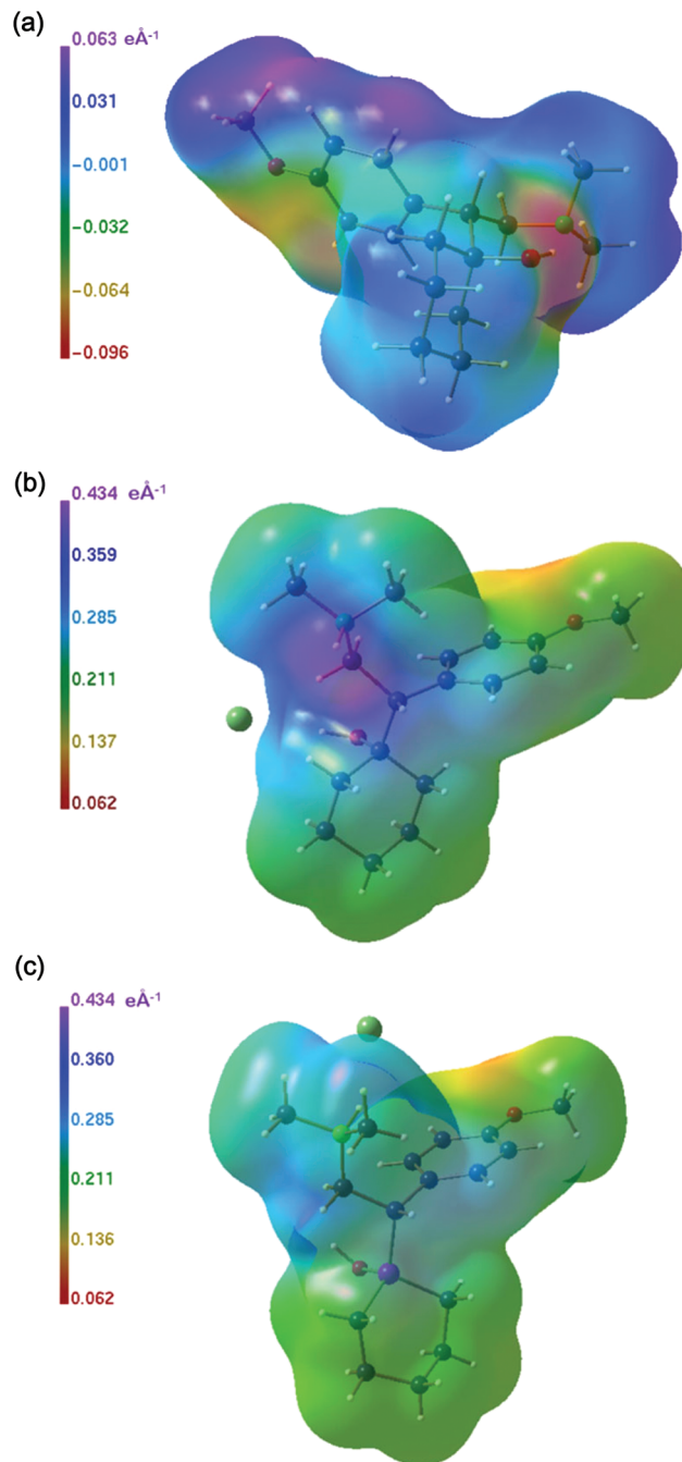
Fig. 9 Electrostatic potentials of 2a (a), 2a\cdot\text{HCl-ortho} (b) and 2b\cdot\text{HCl} (c) mapped onto the isoelectron density surface \rho = 0.0067 \text{ e \AA}^{-3} . 31
