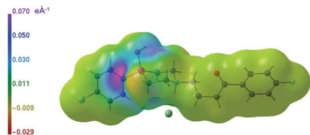
Fig. 8 Electrostatic difference potential 1b\cdot\text{HCl}/1a\cdot\text{HCl} . 31
