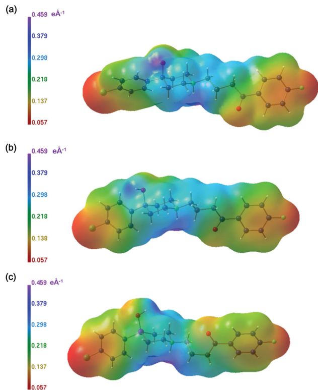
Fig. 7 Electrostatic potentials of the ammonium cations of 1a\cdot\text{HCl} (a), 1a\cdot\text{HPic} (b) and 1b\cdot\text{HCl} (c) mapped onto the isoelectron density surface \rho = 0.0067 \text{ e \AA}^{-3} . 31
