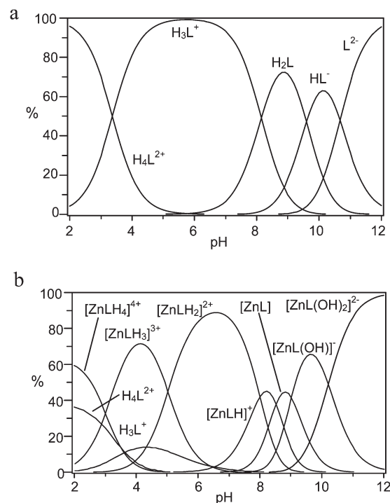
Fig. 1 Distribution diagrams of (a) the protonated species, and (b) the \text{Zn}(\text{II}) complexes formed by receptor 1 ( \text{L}^{2-} , \text{NMe}_4\text{Cl} , 0.1 M, 308 K).
