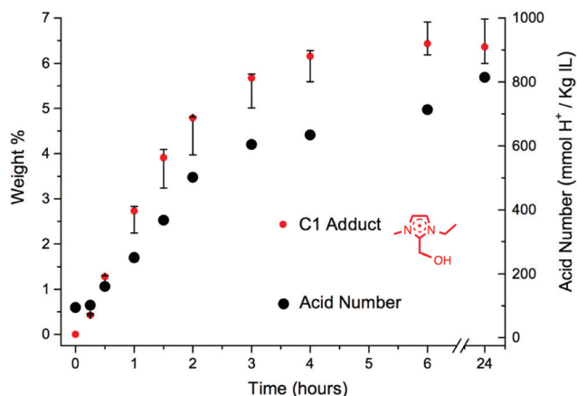
Fig. 7 Relationship between acid number and wt% of the C1 adduct, [C 2 C 1 (HO)C 1 2 im] + , for the mixture of [C 2 C 1 im][OAc], 1a + 10 wt% D-(+)-glucose, 12 , heated at 120 °C for 24 hours.
