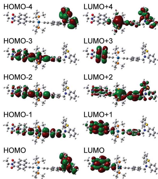
Fig. 12 Orbitals involved in the major electronic transitions of 1 (see Table 3).
