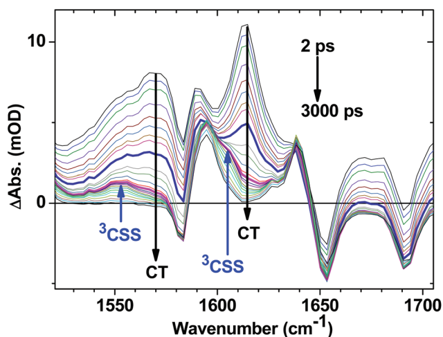
Fig. 6 Expanded fingerprint region of the TRIR data for 1 (Fig. 5d) with delay times spanning from 2 ps to 3 ns following 400\text{ nm} , \sim 50\text{ fs} excitation. Arrows indicate the bands associated with the decay of the CT state, and grow in of ^3\text{CSS} . The highlighted spectra are at delay times of 10 ps (thick blue) and 45 ps (magenta); the latter contains the most pronounced features of ^3\text{CSS} .
