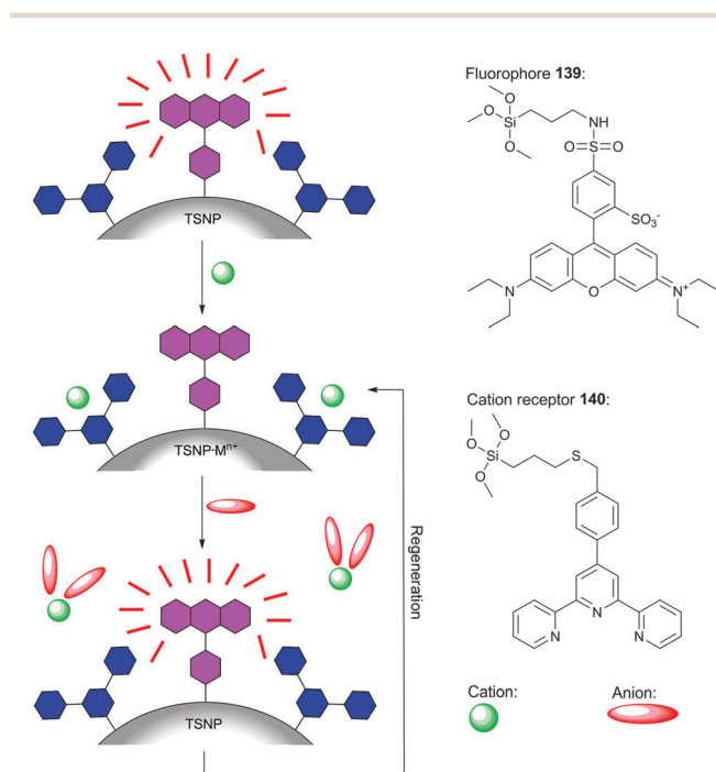
Scheme 17 Design concept of the anion quencher displacement assay (QDA) involving terpyridine-sulforhodamine functionalised nanoparticle (TSNP) and a metal ion quencher, along with the structure of fluorescent dye 139 (magenta) and cation receptor 140 (blue).
