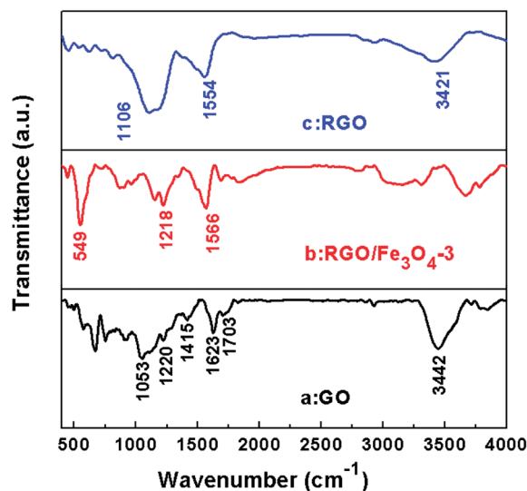
Fig. 4 FT-IR spectra of GO (a), the \text{RGO-Fe}_3\text{O}_4 -3 composite (b) and RGO (c).
